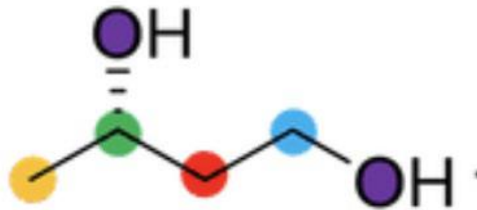
Molecular structure
